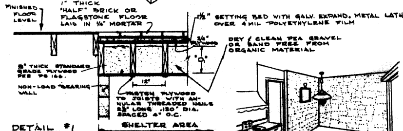
DETAIL #1 SHELTER CEILING CONSTRUCTION WHEN BRICK IS USED
