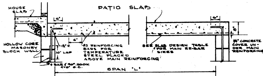
PATIO SLAB AND ANCHORAGE DETAIL
