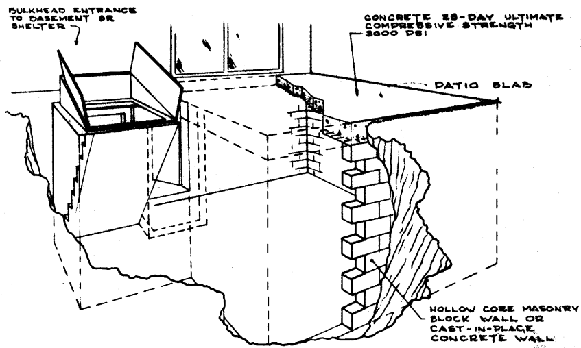
PATIO SLAB AND ANCHORAGE DETAIL
