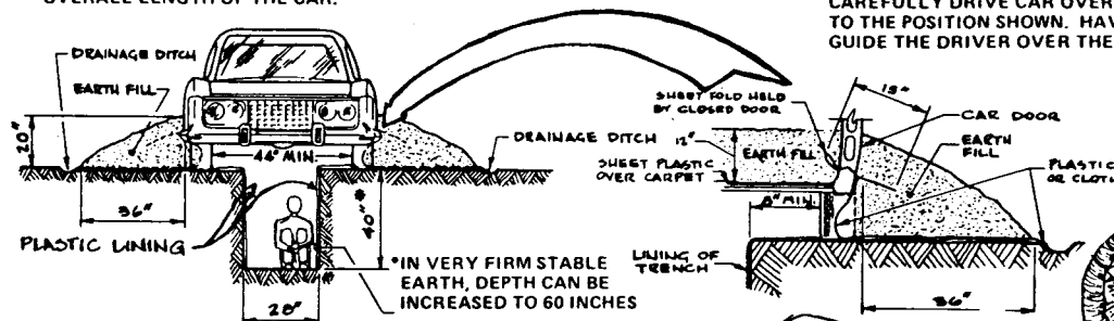
TRENCH AND FILL DETAIL
