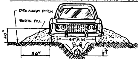
TRENCH AND FILL DETAIL
