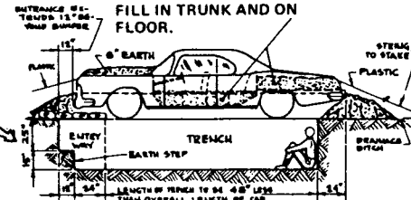
TRENCH AND ENTRYWAY DETAIL
