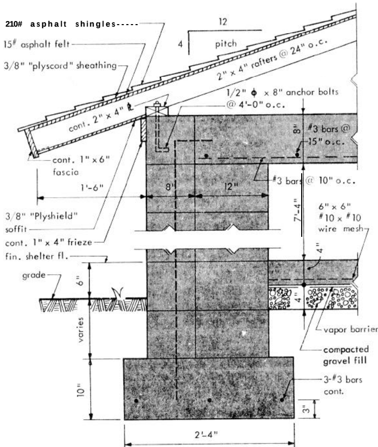
SECTION C-C
