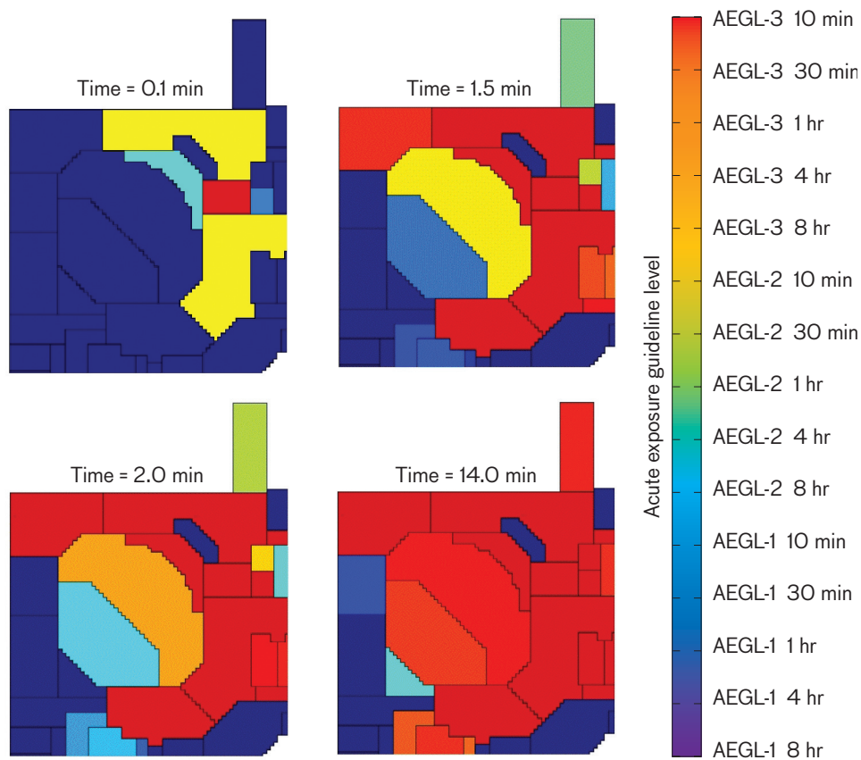
FIGURE 5. The auditorium and prefuction areas show high concentrations of sarin resulting from 1 kg release in the prefuction area. Without any protective measures, the entire prefuction area is contaminated to a lethal dose (acute exposure guideline limit AEGL-3 stages) within two minutes, and the auditorium within fourteen minutes.
