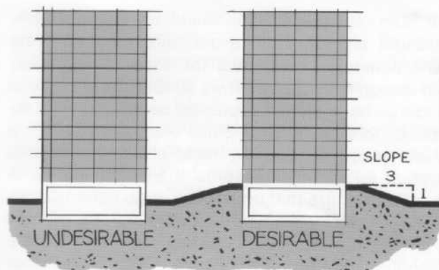
EARTH BERMS INCREASE BOTH BLAST AND FALLOUT PROTECTION
