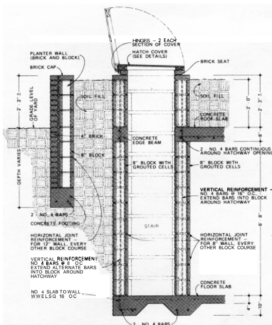
SECTION C - C AT HATCHWAY
