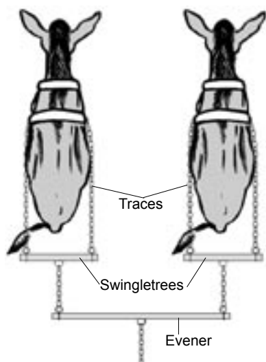
Fig. 18: Two animals hitched abreast. Evener for use with two animals
