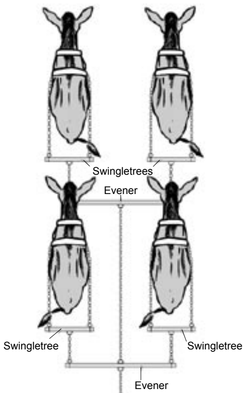
Fig. 21: Four animals hitched in tandem for pulling field implements
