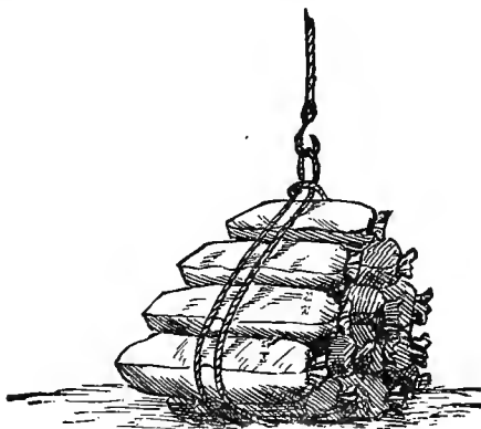
Fig. 182.—ENDLESS ROPE-SLING.
