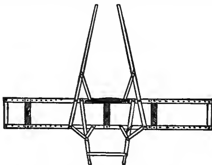
Fig. 56.—LAND-MARKER COMPLETE.
