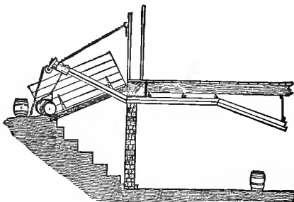
Fig. 183.—A CELLAR CARRIER.
