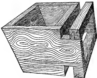
Fig. 6.—FENCE FEED BOX.
