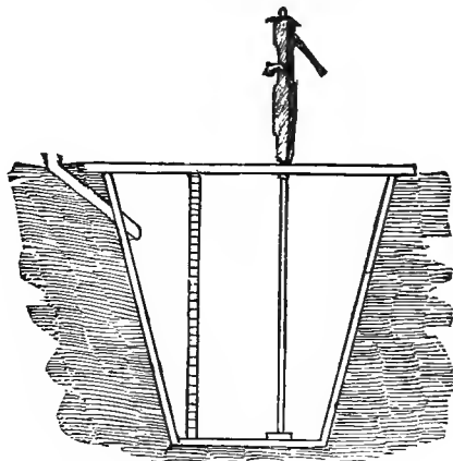
Fig. 143.—A COMPLETE CISTERN.
