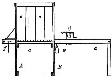
Fig. 167.—THE COMPLETE MACHINE (STRAW-TWISTER).
