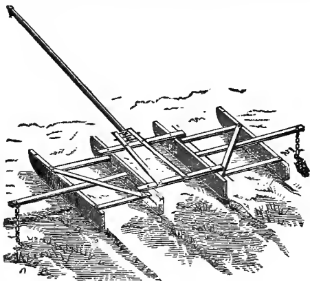
Fig. 59.—A HORSE LAND-MARKER.
