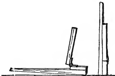
Fig. 39.—WAGON-JACK.
