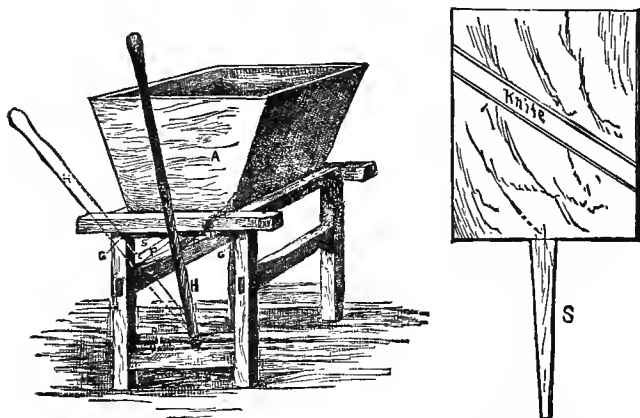
Fig. 86.—HOME-MADE ROOT-CUTTER. Fig. 87.—ROOT-CUTTER SLIDE.
