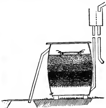
Fig. 141. A SERVICEABLE FILTER.
