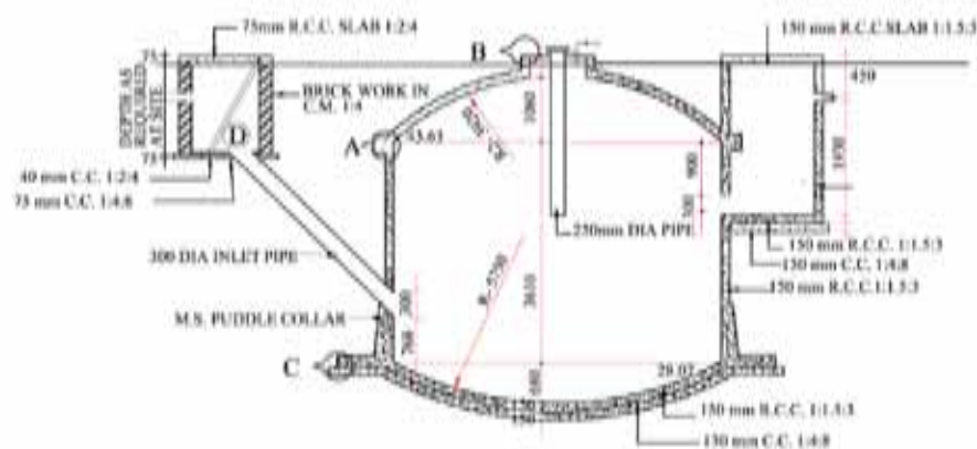
SECTIONAL ELEVATION
