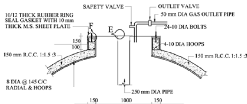
DETAIL AT B
