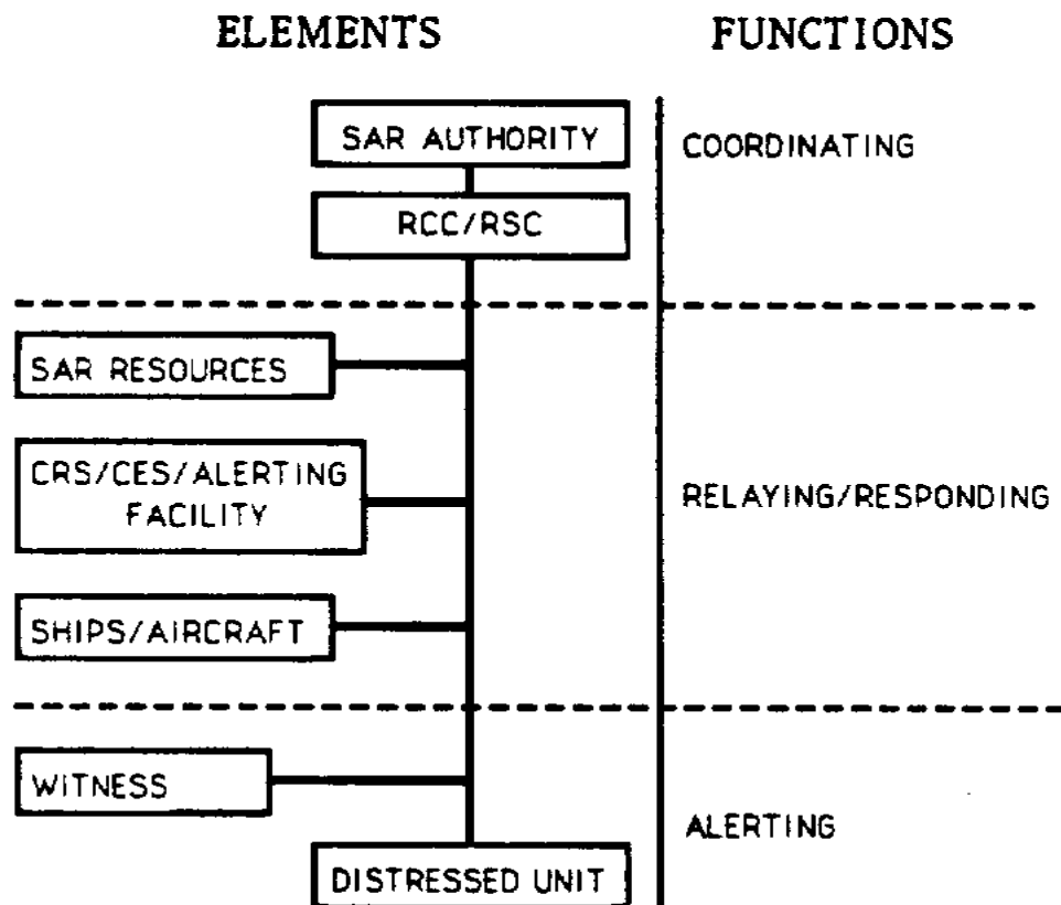
Figure 1-1. SAR System 1
