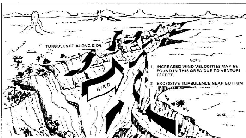
Figure 8-2. Wind Flow in Valley or Canyon
