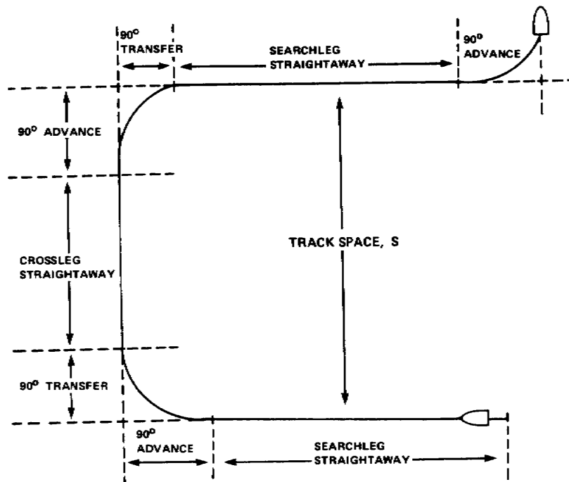
Figure 6-6. Marine SRU Crossleg Figure 6-6. Marine SRU Crossleg
