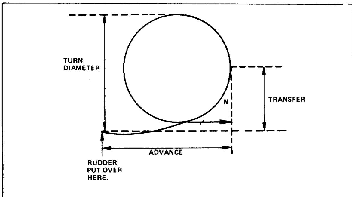
Figure 6-7. Typical Vessel-Turning Circle Figure 6-7. Typical Vessel-Turning Circle
