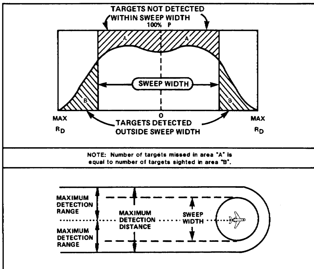
Figure 5-16. Sweep Width
