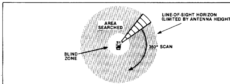
Figure 6-13. Surface Vessel Radar (SVR)
