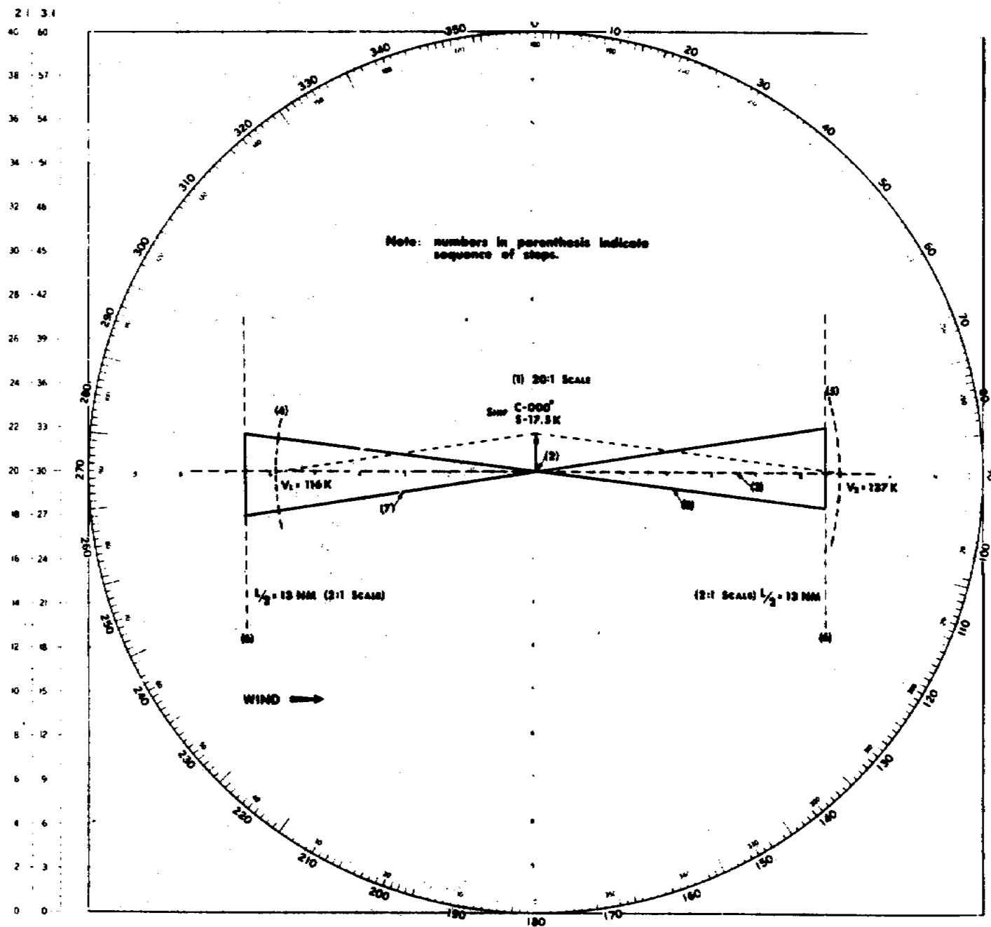
Figure E-6. Geometric Solution of Relative Motion Pattern
