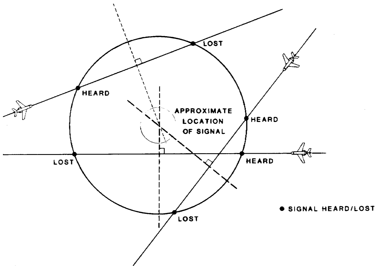
Figure 6-5. Search for EPIRB/ELT Figure 6-5. Search for EPIRB/ELT
